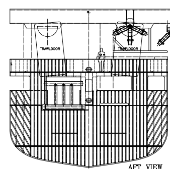
AFT VIEW
