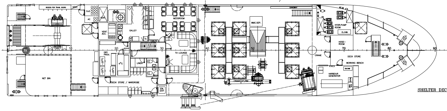
FORECASTLE DECK
