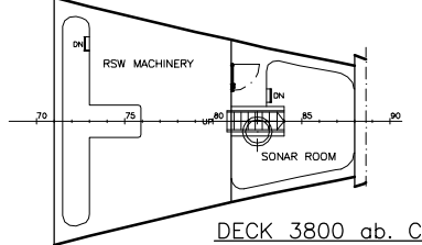
2.nd. DECK
