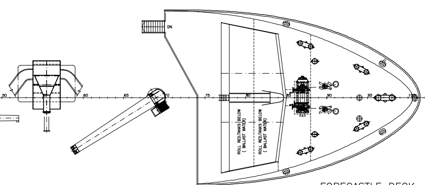
FORECASTLE DECK
