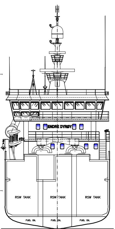
MIDSHIP SECTION
