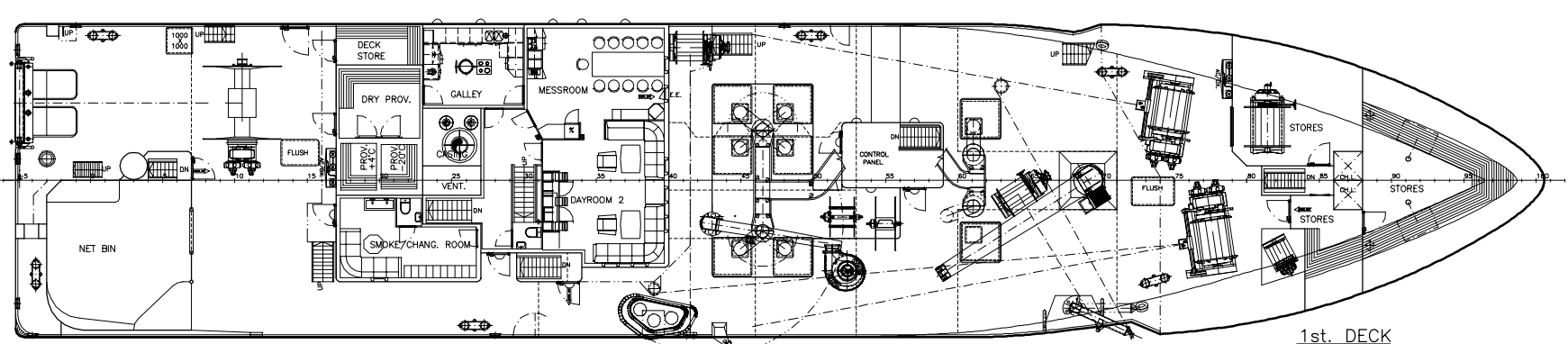
1st. DECK
