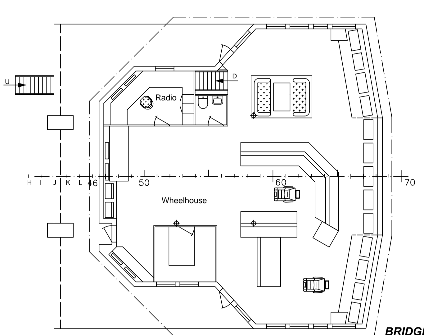
BRIDGE DECK
