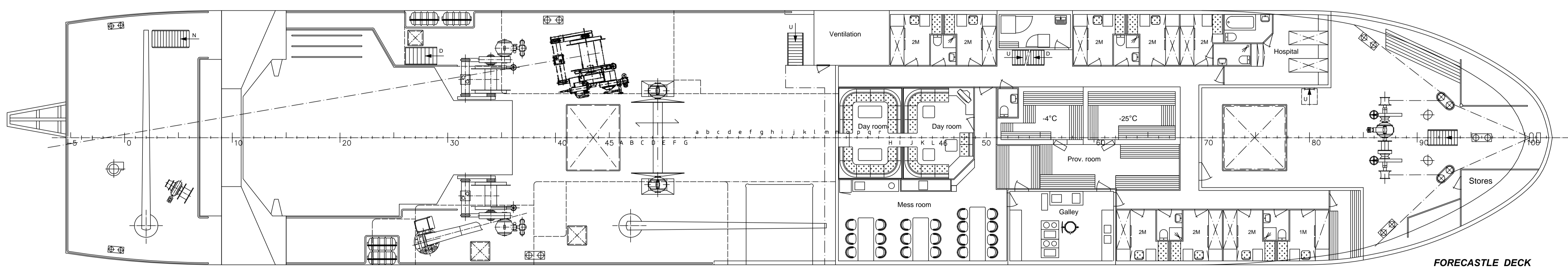
FORECASTLE DECK
