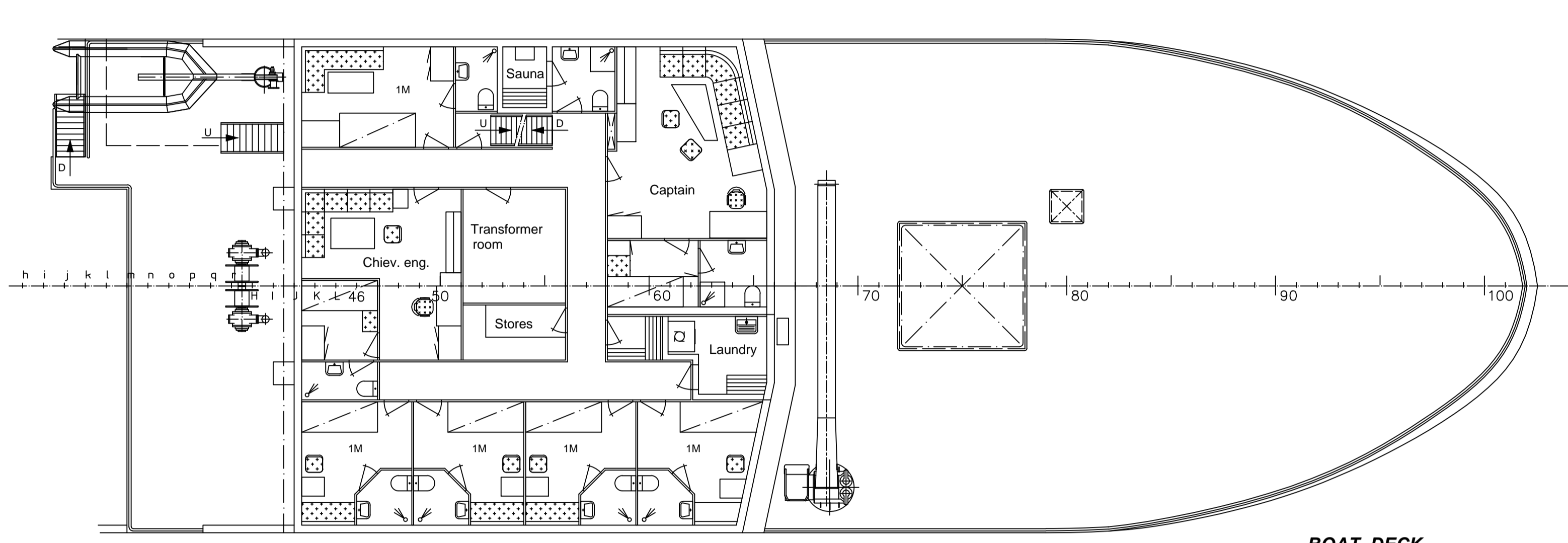
BOAT DECK
